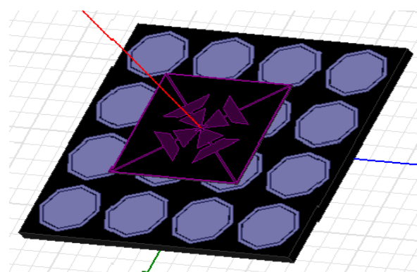
Fig. 1(a): Proposed antenna
