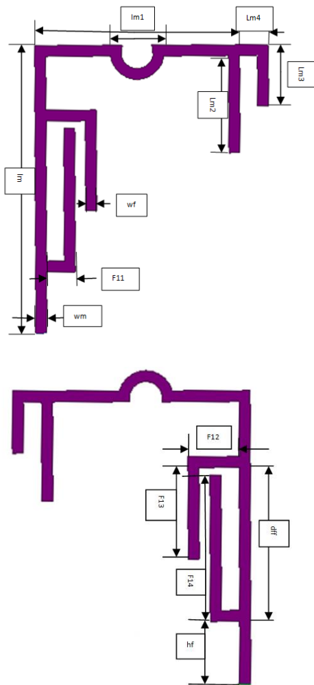
Fig.2: Feeding structures of antenna
