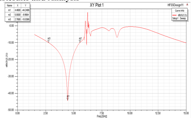
Fig. 4(a): Simulated result for bandwidth of proposed antenna
