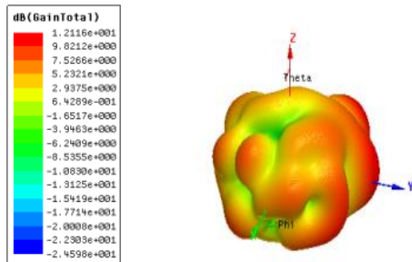
Fig. 5(a): Gain of the proposed antenna Radiation Pattern 1
